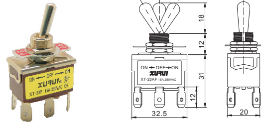
• 双极双向自动复位型 DPDT Auto Reset (ON)-OFF-(ON) XT-23AF
