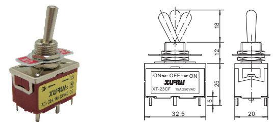
• 双极双向自动复位型 DPDT Auto Reset (ON) -OFF-(ON) XT-23CF
